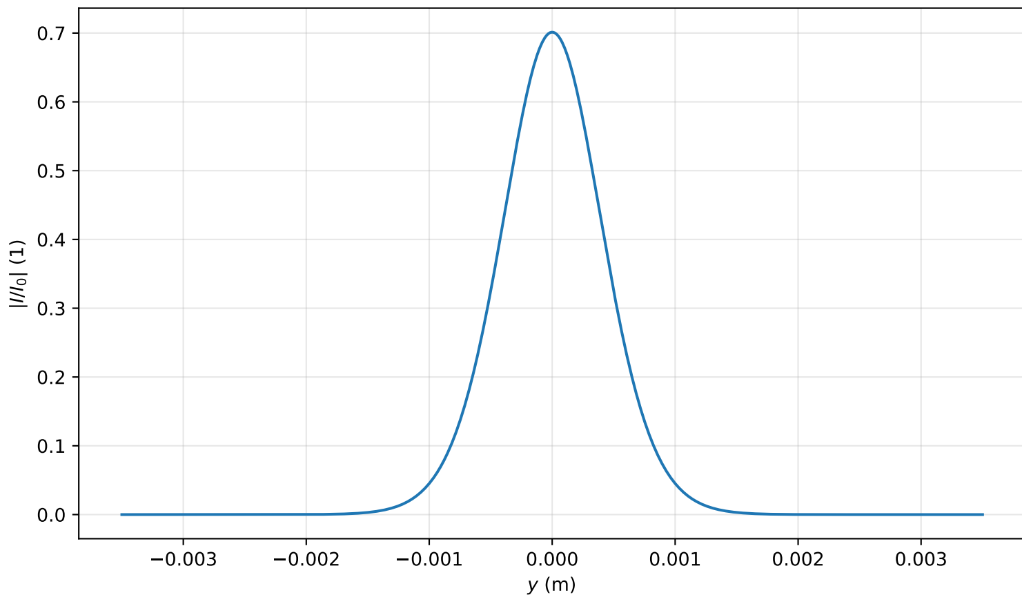
Intensity profile I(x=0, y, z=1.831)/I_0 , P_{in}=0.3P_{cr} , artificial time
